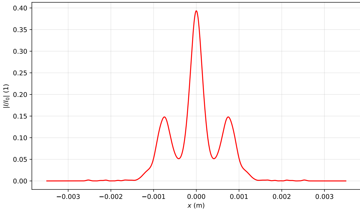
Intensity profile I(x, y = 0, z = 1.911)/I_0 , P_{in}=7.5P_{cr} , artificial time
